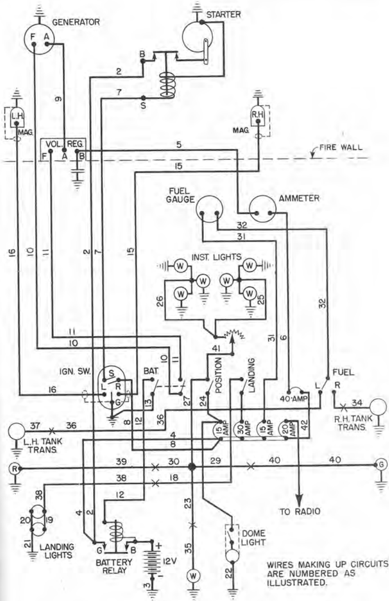
Figure 57—Electrical Wiring Diagram (Models 108, -1, -2)
