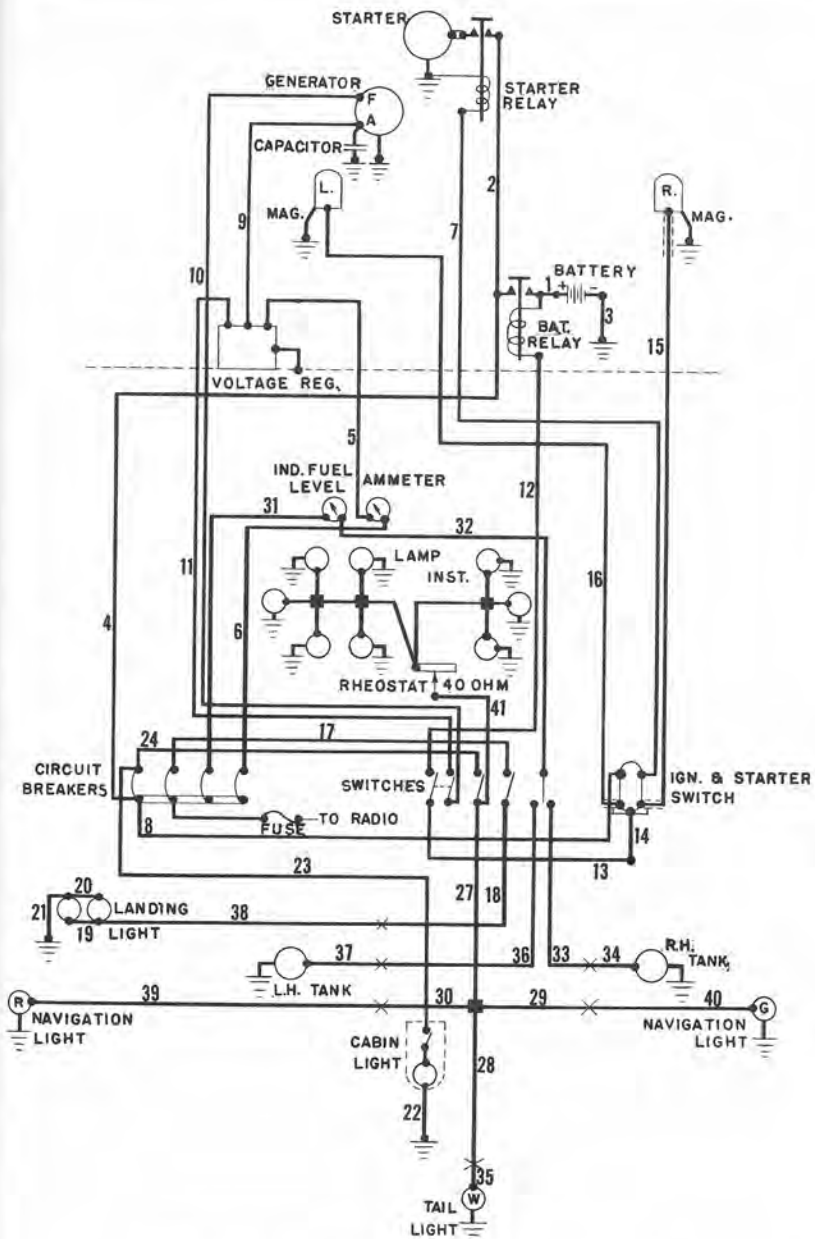
Figure 59—Electrical Wiring Diagram (Model 108-3)
